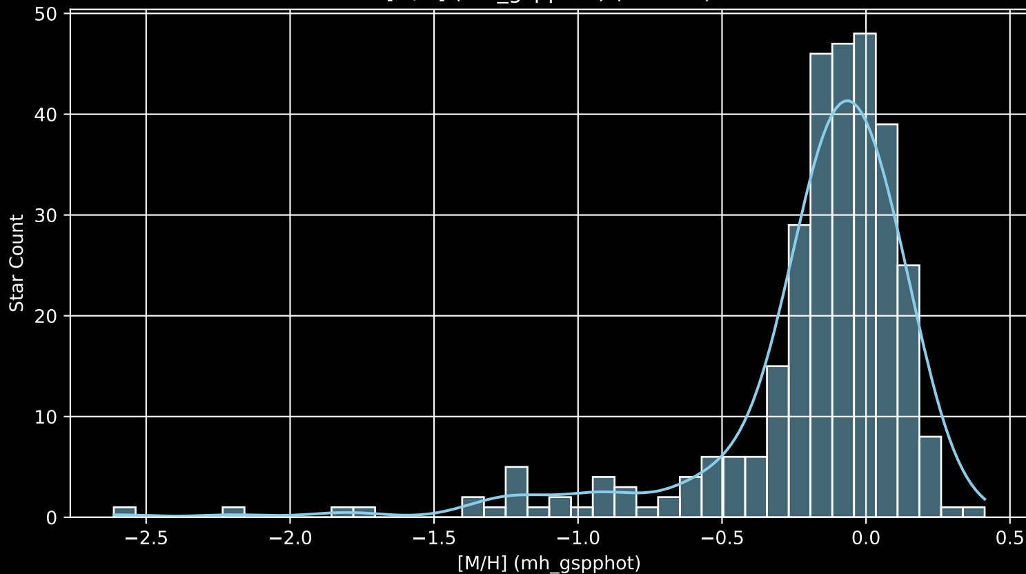
APOGEE DR17 Field: [034-12 [M/H] (mh_gspphot) (n= 307)
