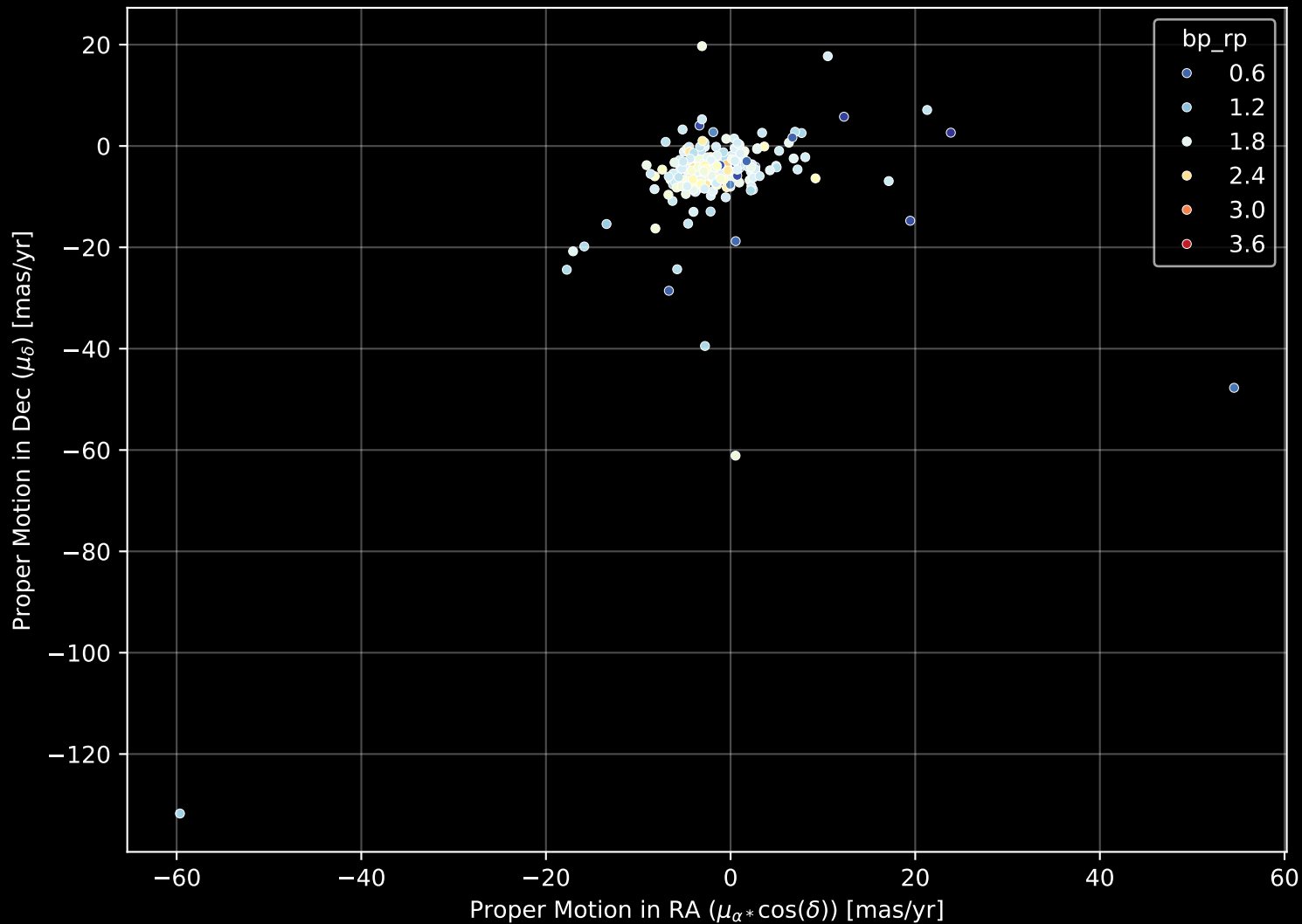
APOGEE DR17 Field: [034-12] Proper Motion Diagram (n= 308)
