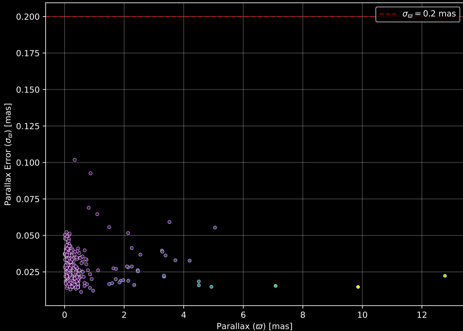
APOGEE DR17 Field: [034-12] Parallax Quality (n= 308)
