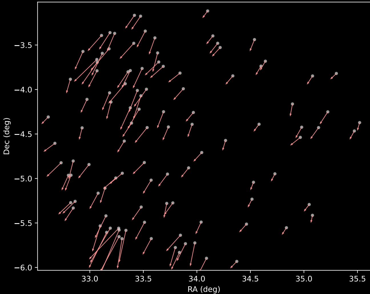
APOGEE DR17 Cluster 7 Proper Motion Vectors (n=107)
