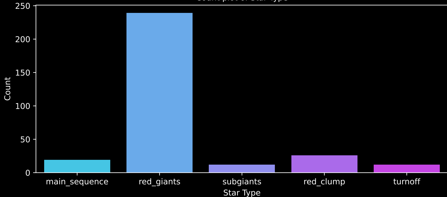
APOGEE DR17 Field: [034-12] Count plot of Star Type
