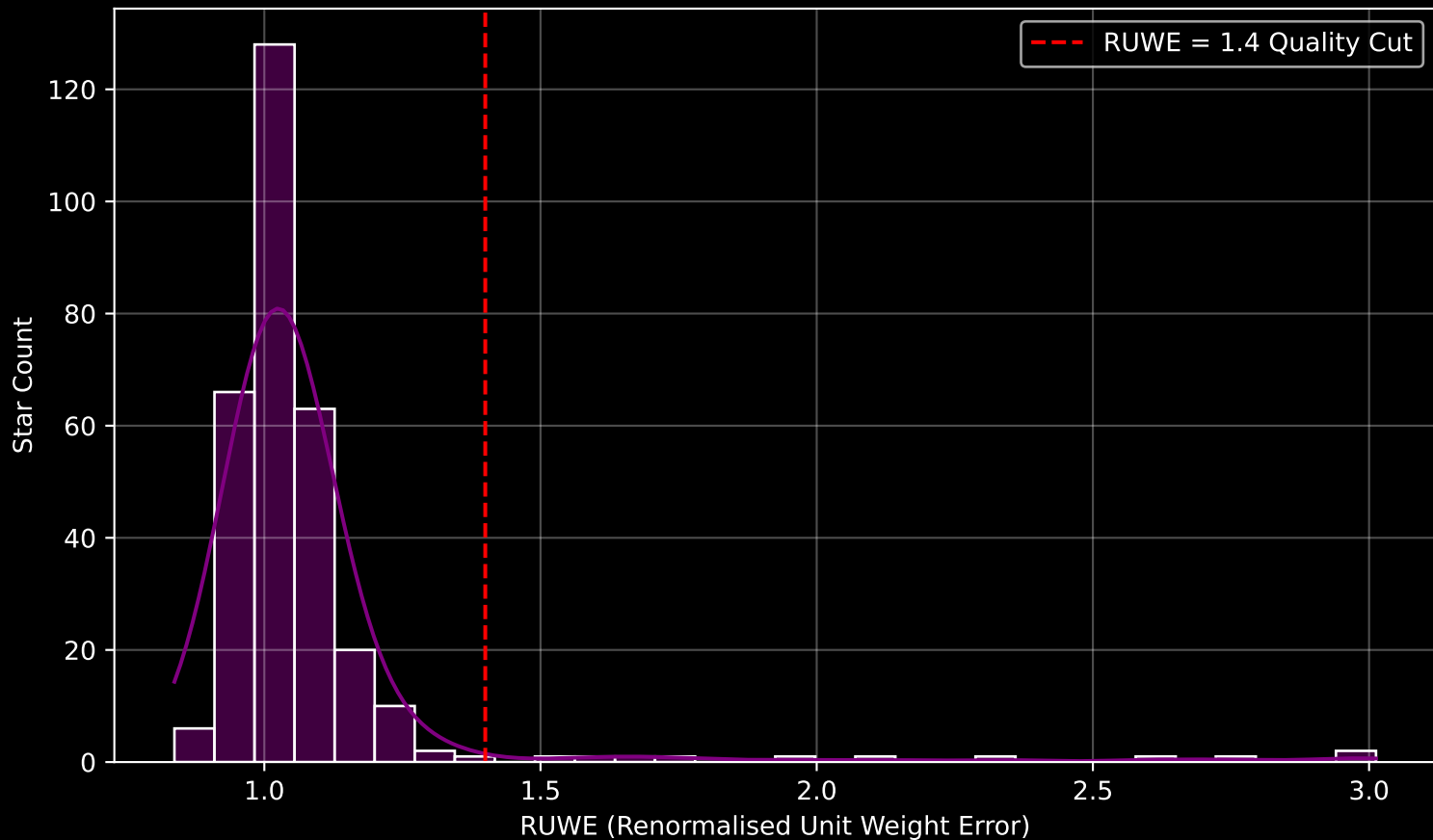
GAPOGEE DR17 Field [034-12] RUWE Distribution (n= 307)
