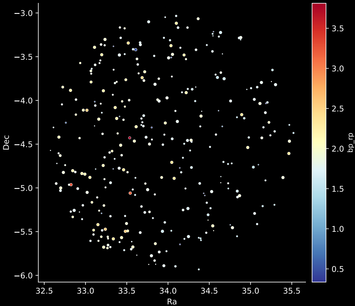
APOGEE DR17 Field: [034-12] Stars: 308
