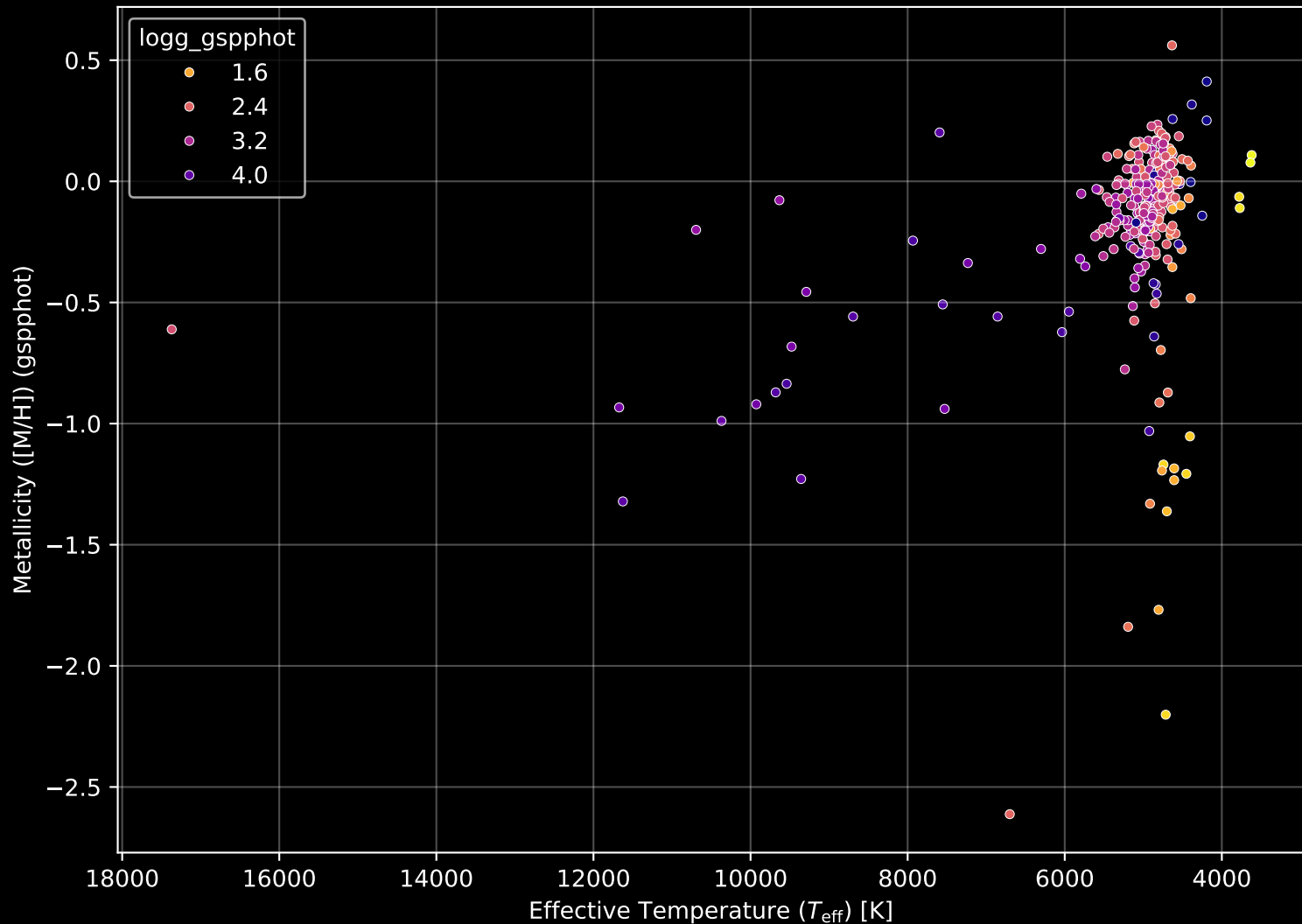
APOGEE DR17 Field: [034-12] Stellar Population Parameters (n= 308)
